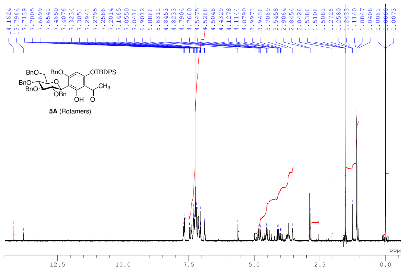
^1\text{H} NMR spectrum of 5A in \text{CDCl}_3 (500 MHz)
