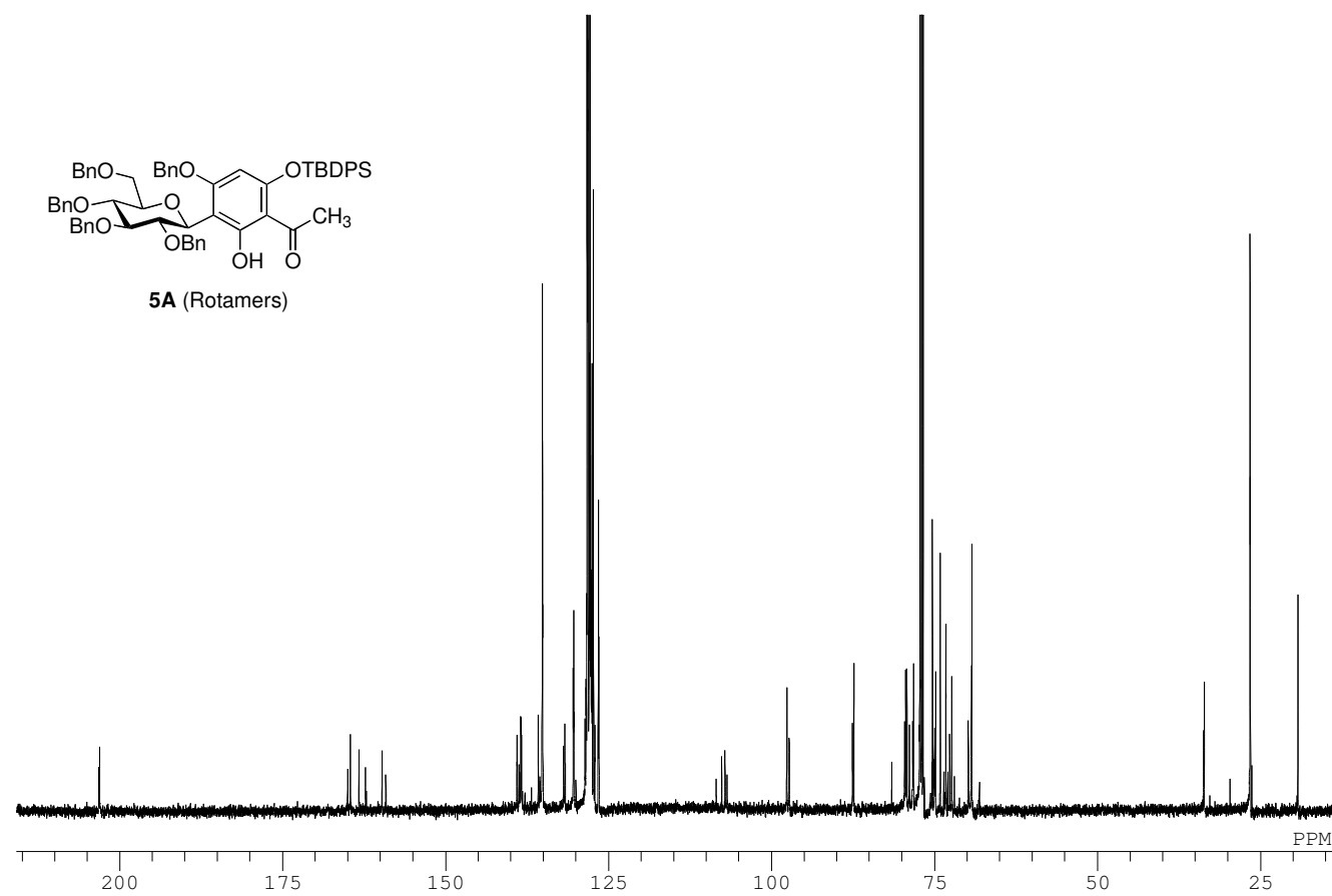
^{13}\text{C} NMR spectrum of 5A in \text{CDCl}_3 (125 MHz)
