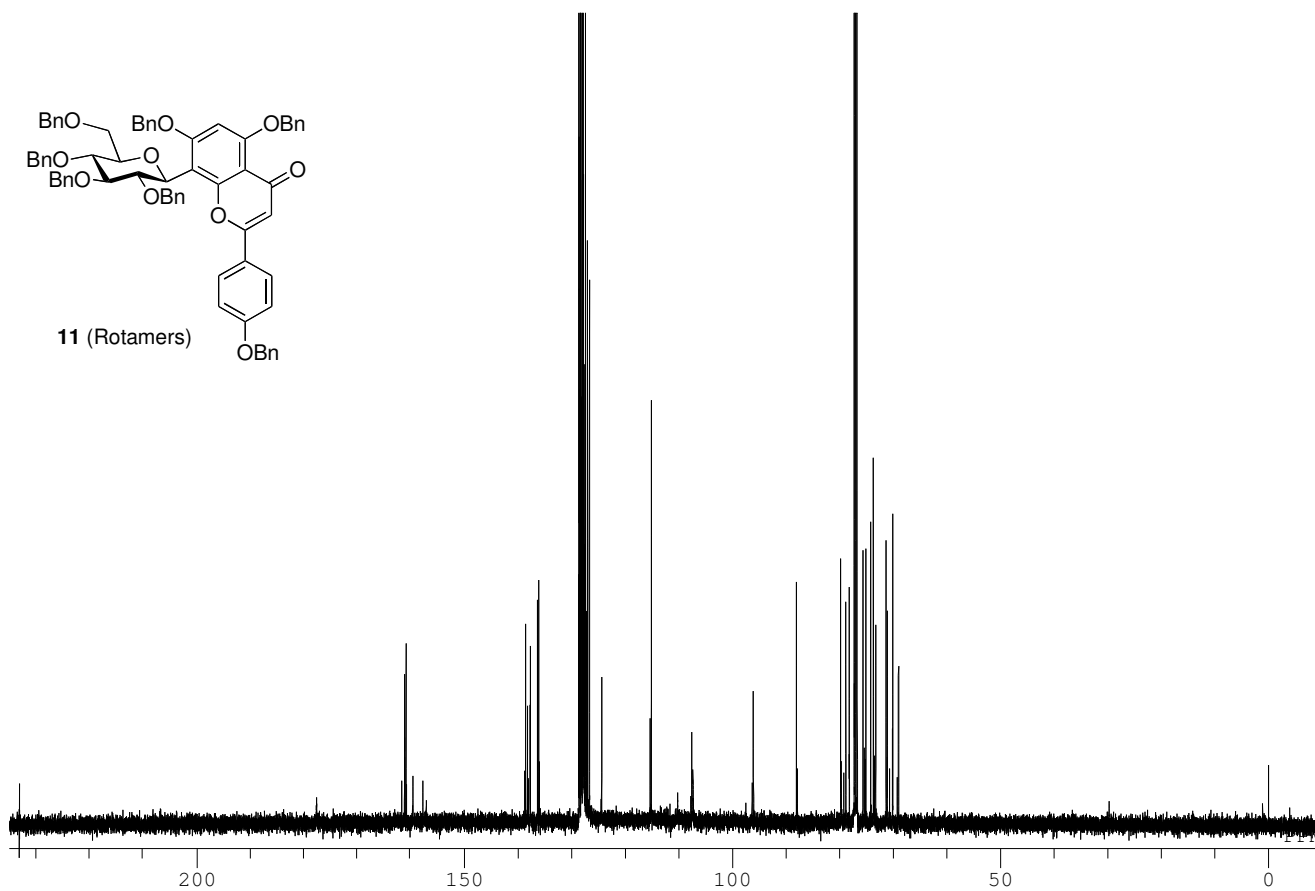
^{13}\text{C} NMR spectrum of 11 in \text{CDCl}_3 (125 MHz)
