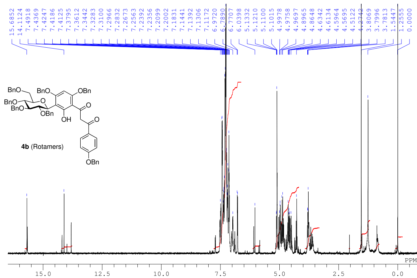
^1\text{H} NMR spectrum of 4b in \text{CDCl}_3 (500 MHz)
