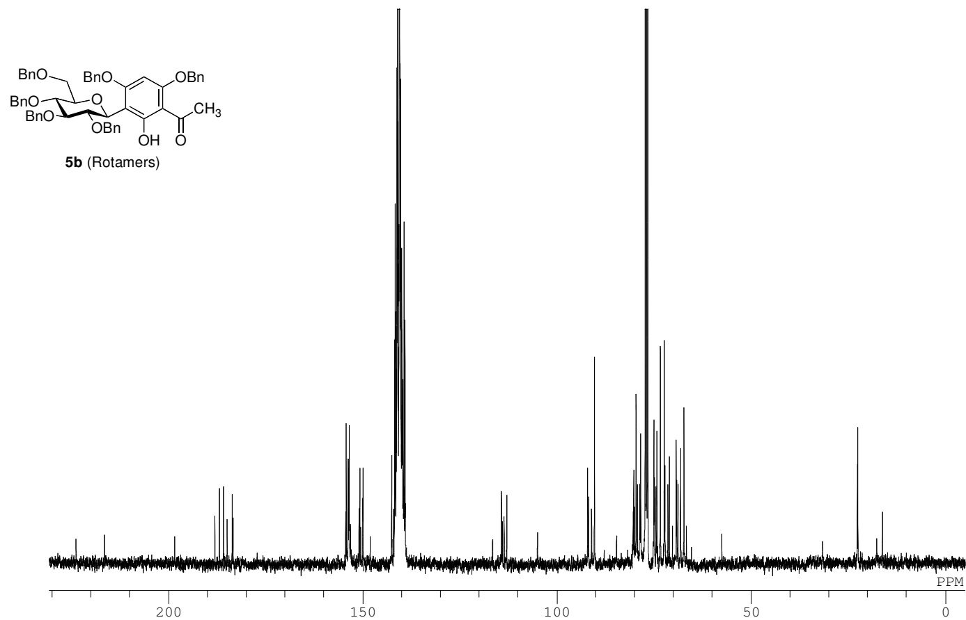
^{13}\text{C} NMR spectrum of 5b in \text{CDCl}_3 (125 MHz)
