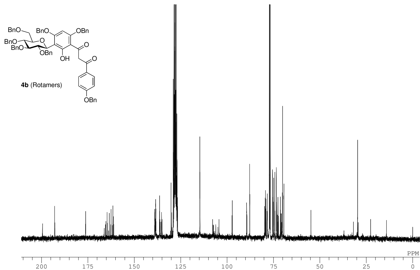
^{13}\text{C} NMR spectrum of 4b in \text{CDCl}_3 (125 MHz)
