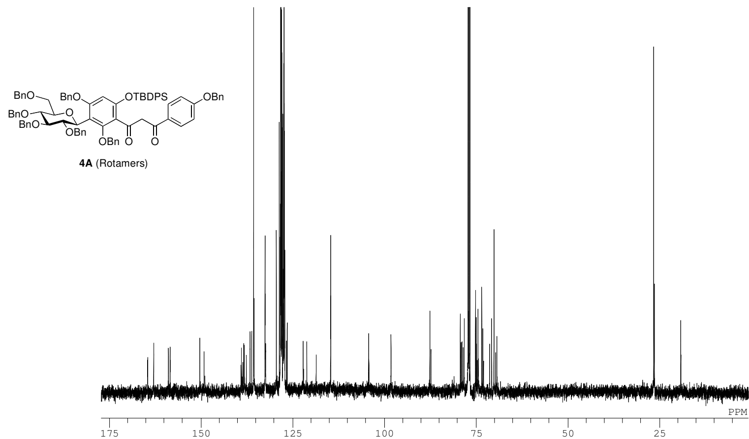
^{13}\text{C} NMR spectrum of 4A in \text{CDCl}_3 (125 MHz)
