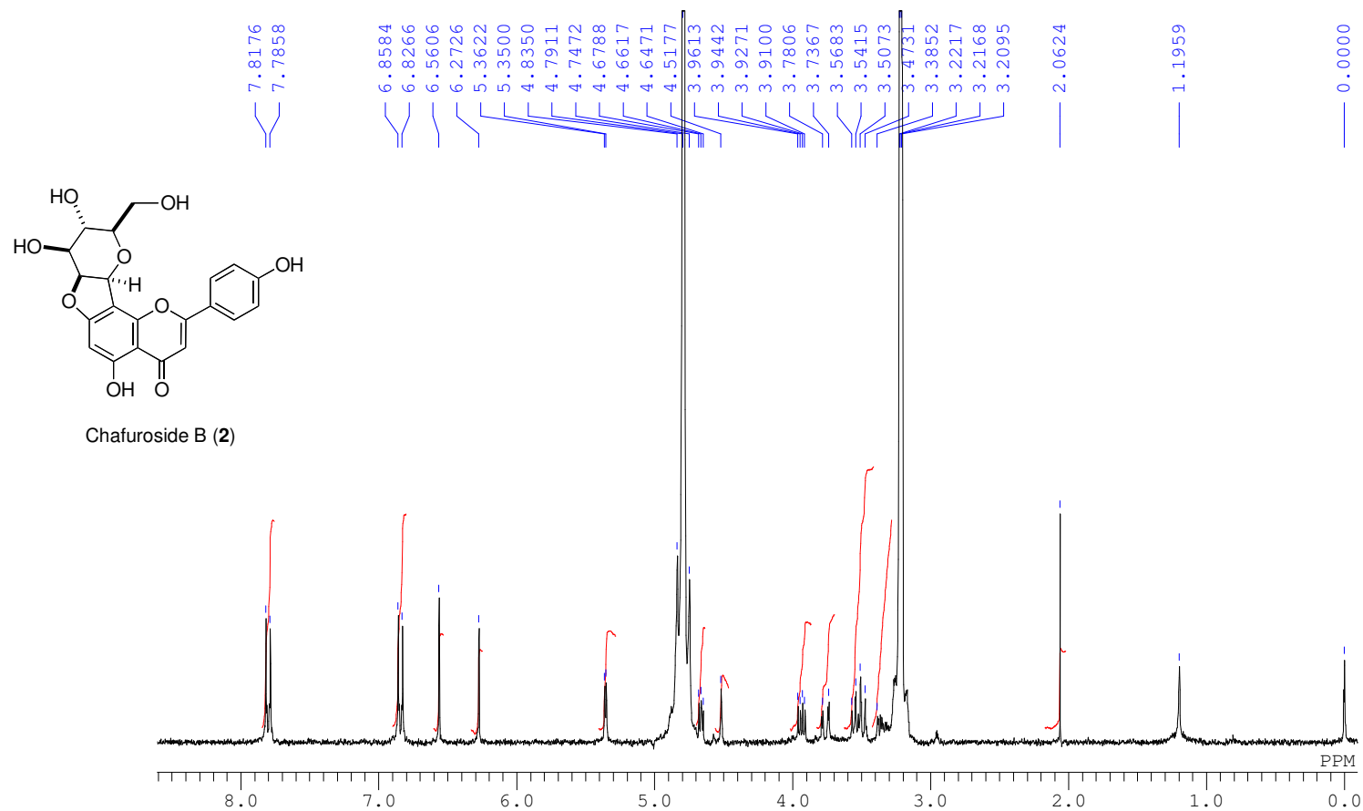
^1\text{H} NMR spectrum of 2 in \text{CD}_3\text{OD} (500 MHz)
