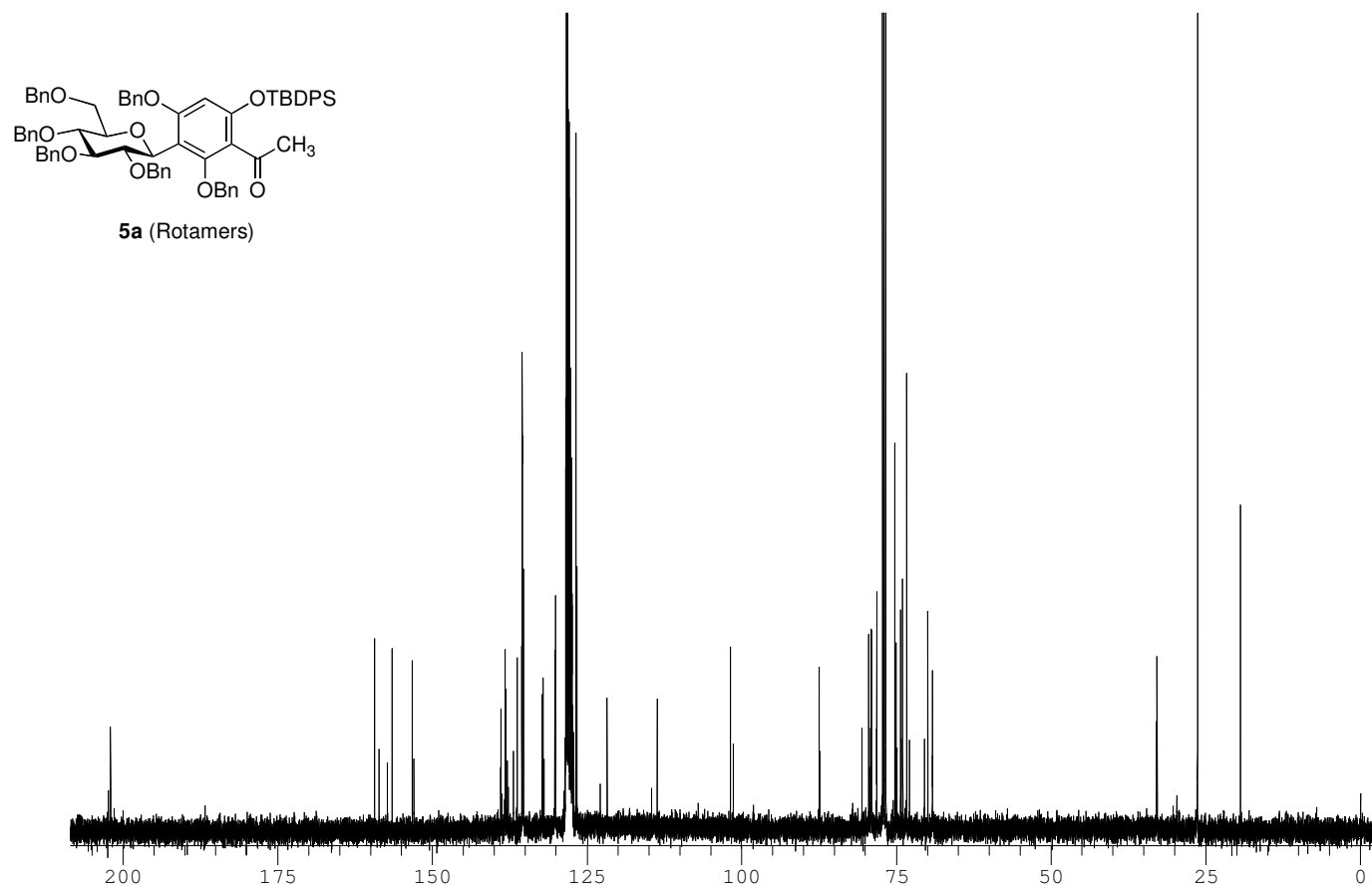
13 C NMR spectrum of 5a in CDCl 3 (125 MHz)
