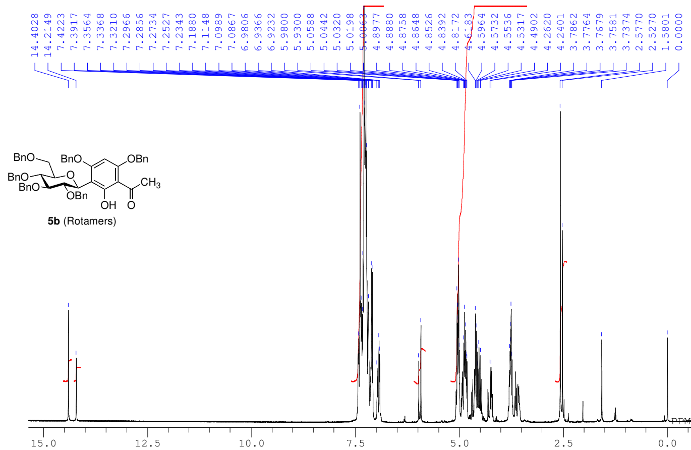
^1\text{H} NMR spectrum of 5b in \text{CDCl}_3 (500 MHz)
