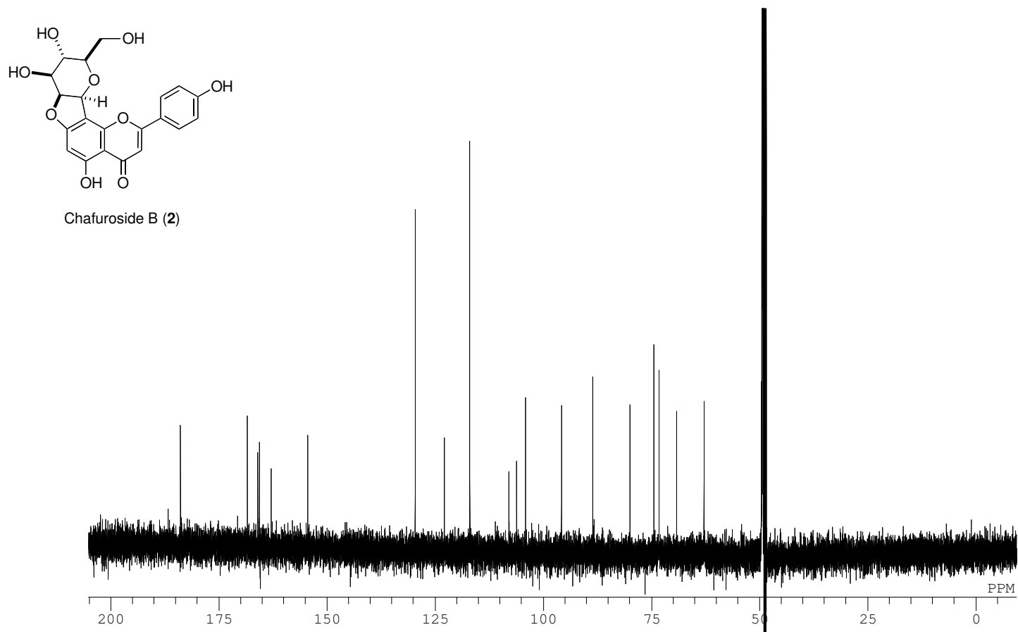
^{13}\text{C} NMR spectrum of 2 in \text{CD}_3\text{OD} (125 MHz)
