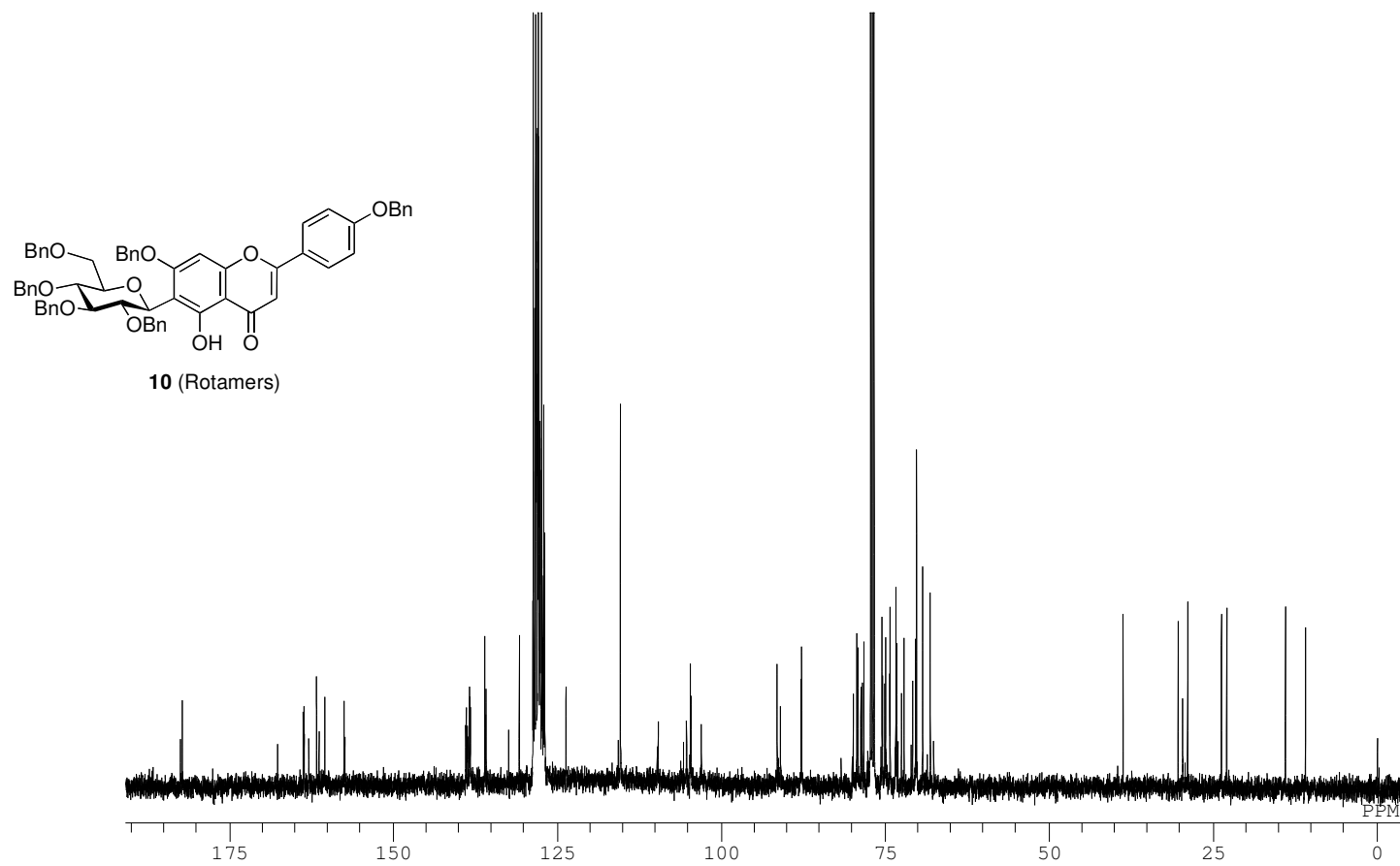
^{13}\text{C} NMR spectrum of 10 in \text{CDCl}_3 (125 MHz)
