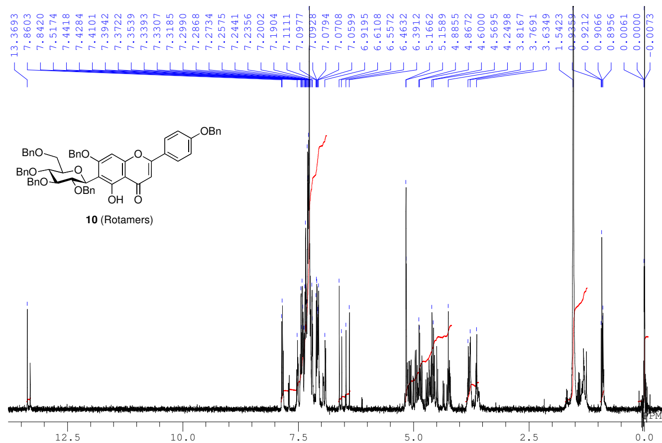
^1\text{H} NMR spectrum of 10 in \text{CDCl}_3 (500 MHz)
