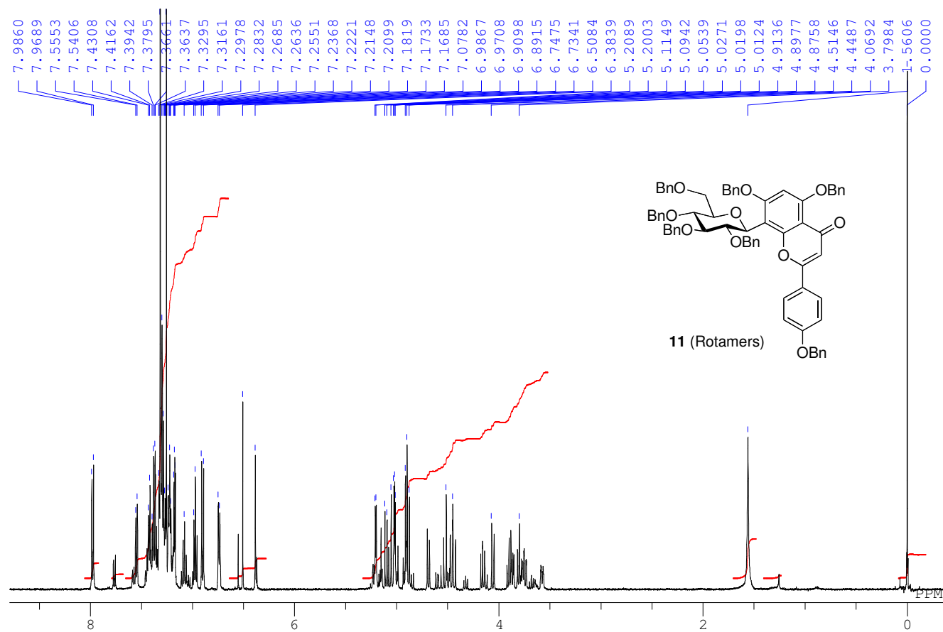
^1\text{H} NMR spectrum of 11 in \text{CDCl}_3 (500 MHz)
