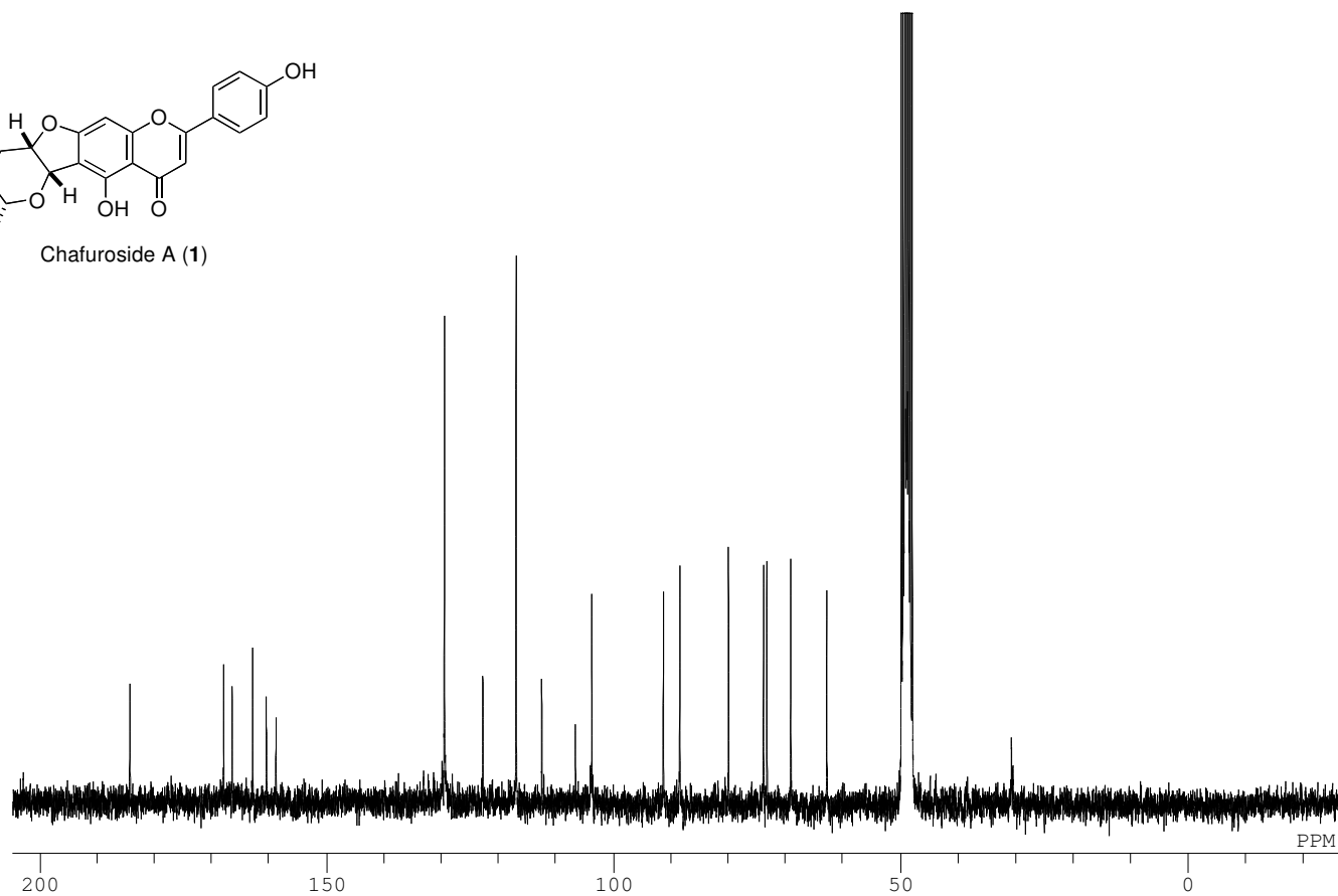
^{13}\text{C} NMR spectrum of 1 in \text{CD}_3\text{OD} (125 MHz)
