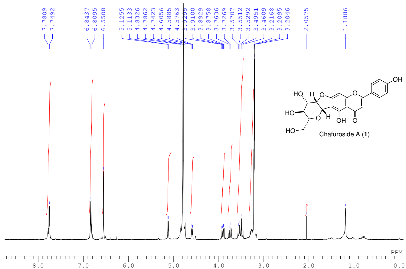
^1\text{H} NMR spectrum of 1 in \text{CD}_3\text{OD} (500 MHz)
