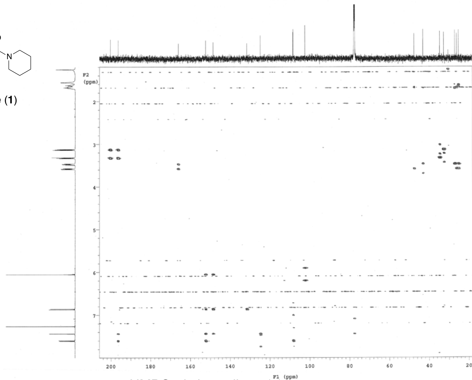
HMBC of piperodione ( 1 )
