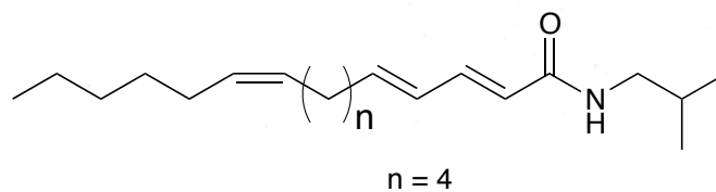
N -isobutyl-(2 E , 4 E , 10 Z )-hexadeca-2,4,10-trienamide ( 3 )
