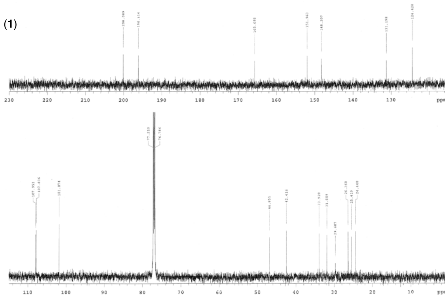
^{13}\text{C} NMR data of piperodione (1)
