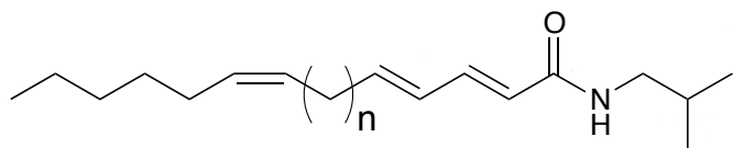
N -isobutyl-(2 E , 4 E , 10 Z )- hexadeca-2,4,10-trienamide ( 3 )
