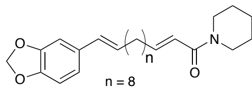
(2 E , 12 E )-pipertridecadienamide ( 2 )
