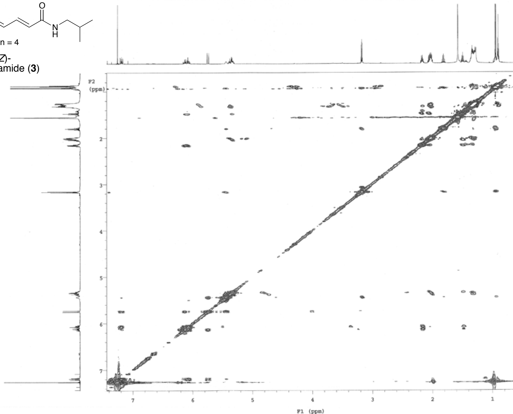
NOESY of N -isobutyl-(2 E , 4 E , 10 Z )-hexadeca-2,4,10-trienamide ( 3 )
