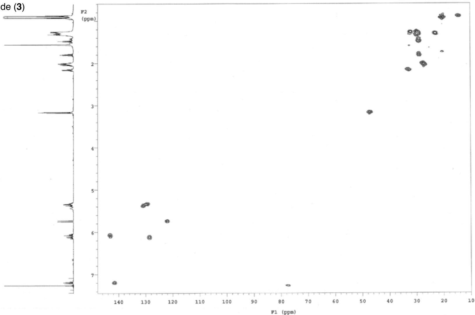
HMQC of N -isobutyl-(2 E , 4 E , 10 Z )-hexadeca-2,4,10-trienamide ( 3 )
