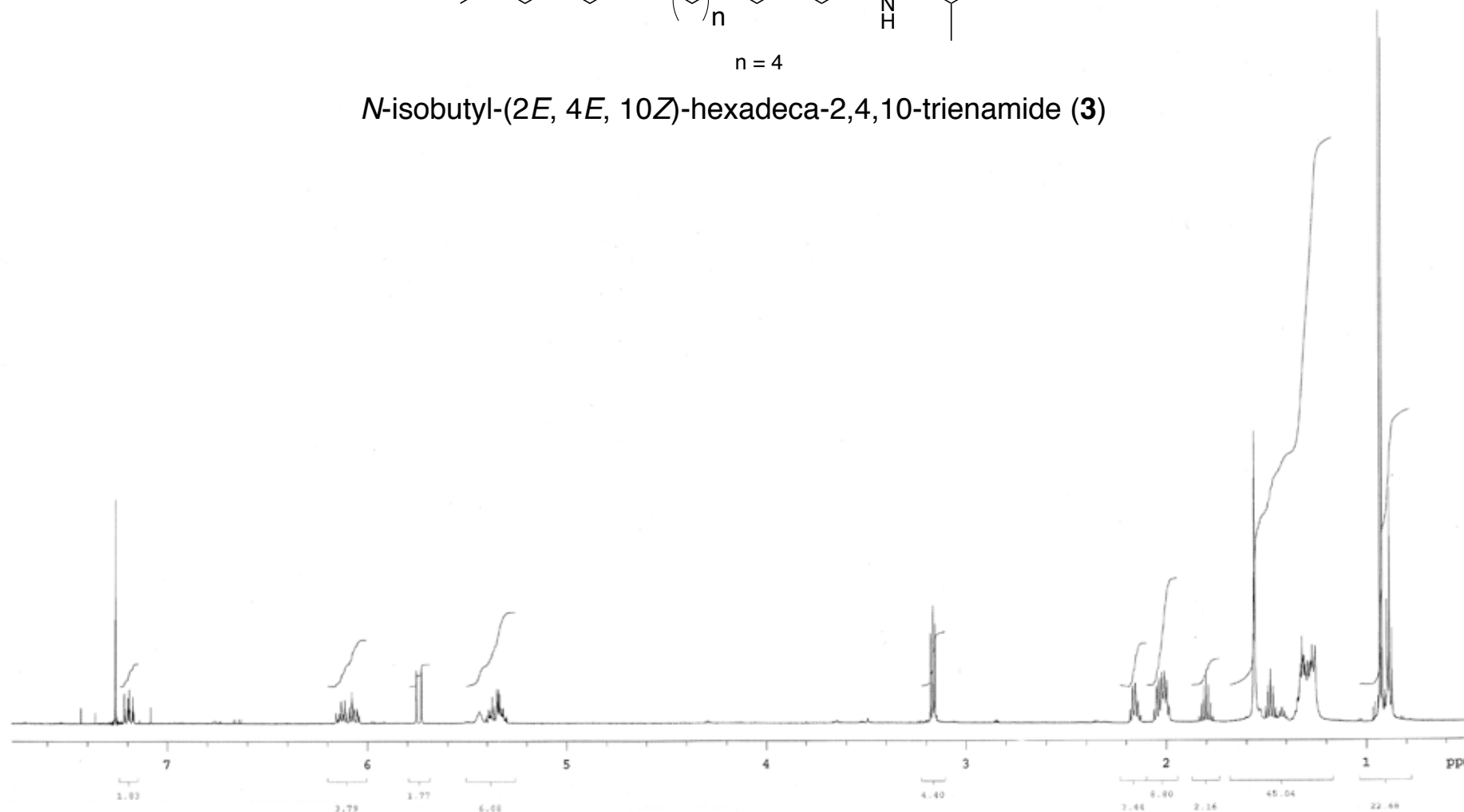
^1\text{H} NMR data of N -isobutyl-(2 E , 4 E , 10 Z )-hexadeca-2,4,10-trienamide ( 3 )
