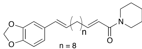
(2 E , 12 E )-pipertridecadienamide ( 2 )
