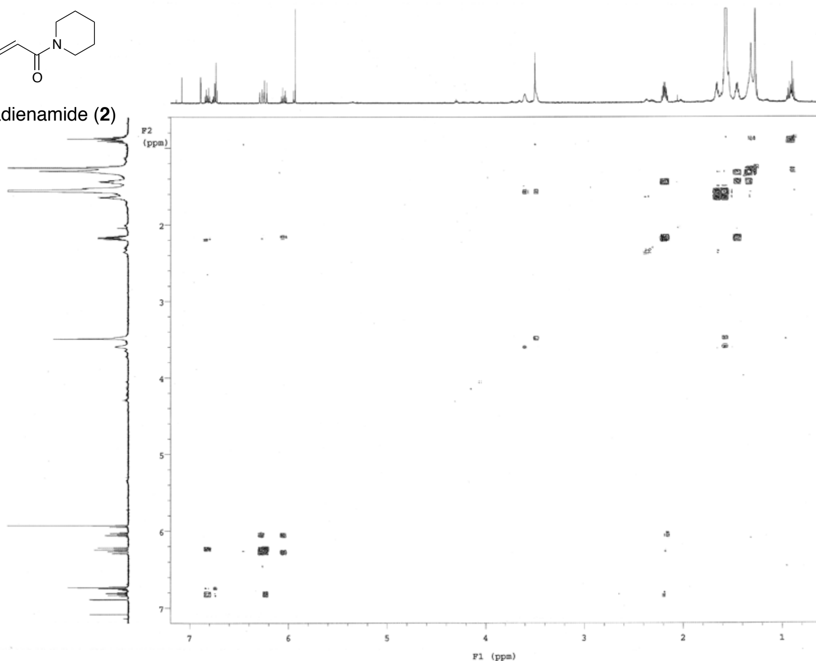
COSY of (2 E , 12 E )-pipertridecadienamide ( 2 )
