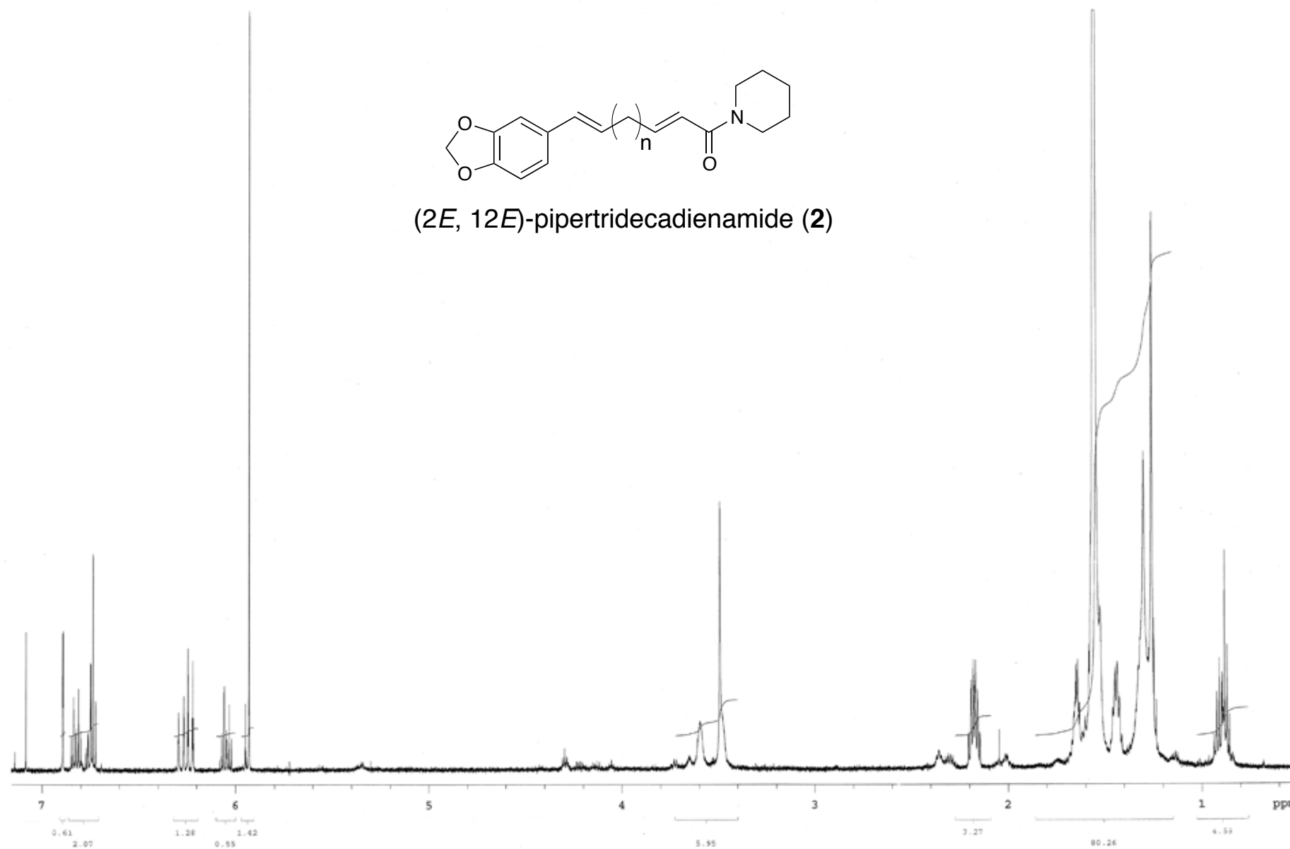
1 H NMR data of (2 E , 12 E )-pipertridecadienamide ( 2 )
