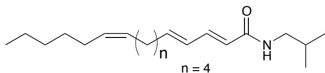
N -isobutyl-(2 E , 4 E , 10 Z )-hexadeca-2,4,10-trienamide ( 3 )
