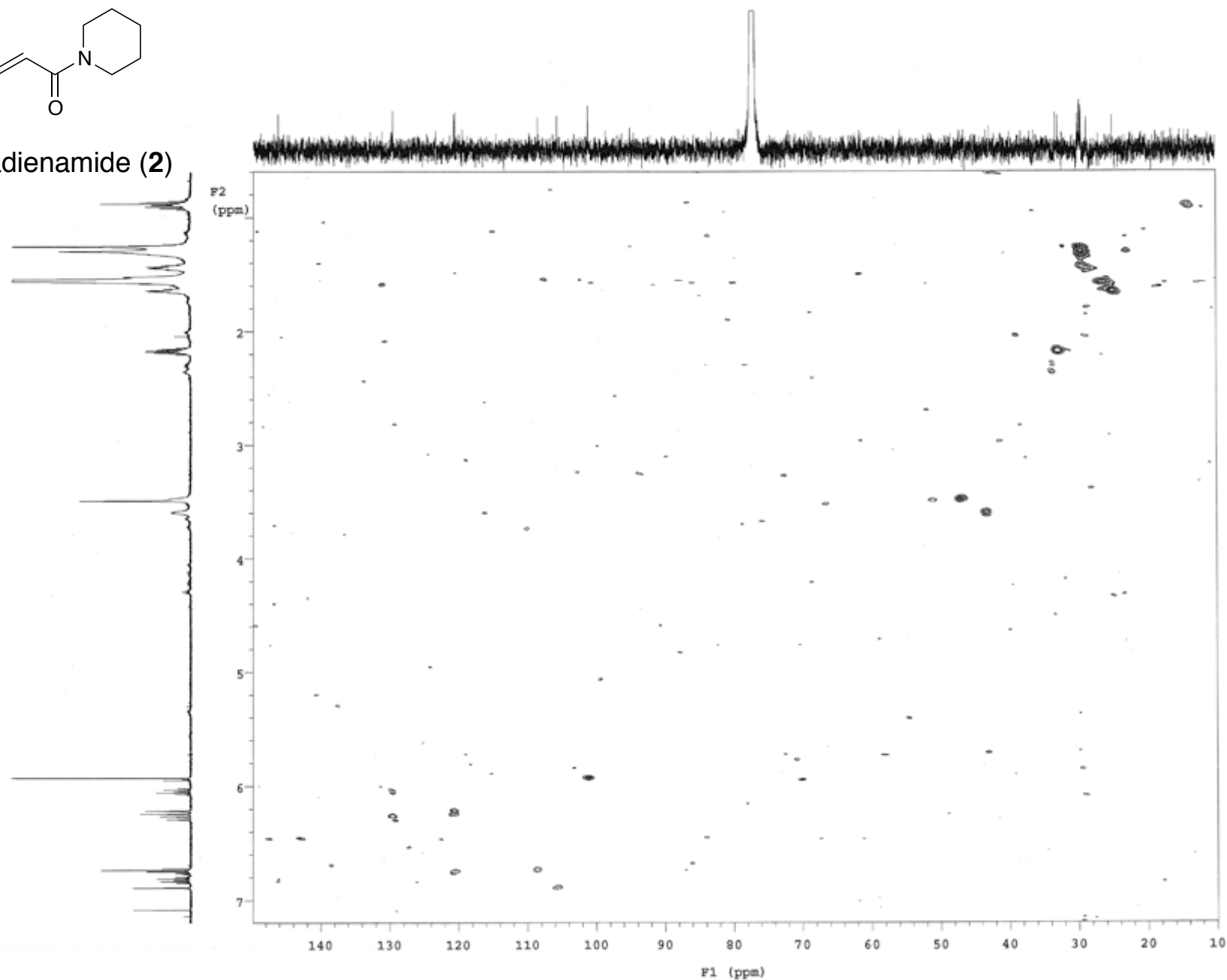
HMQC of (2 E , 12 E )-pipertridecadienamide ( 2 )
