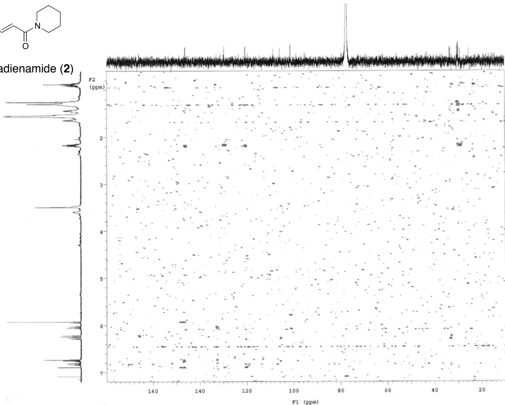
HMBC of (2 E , 12 E )-pipertridecadienamide ( 2 )
