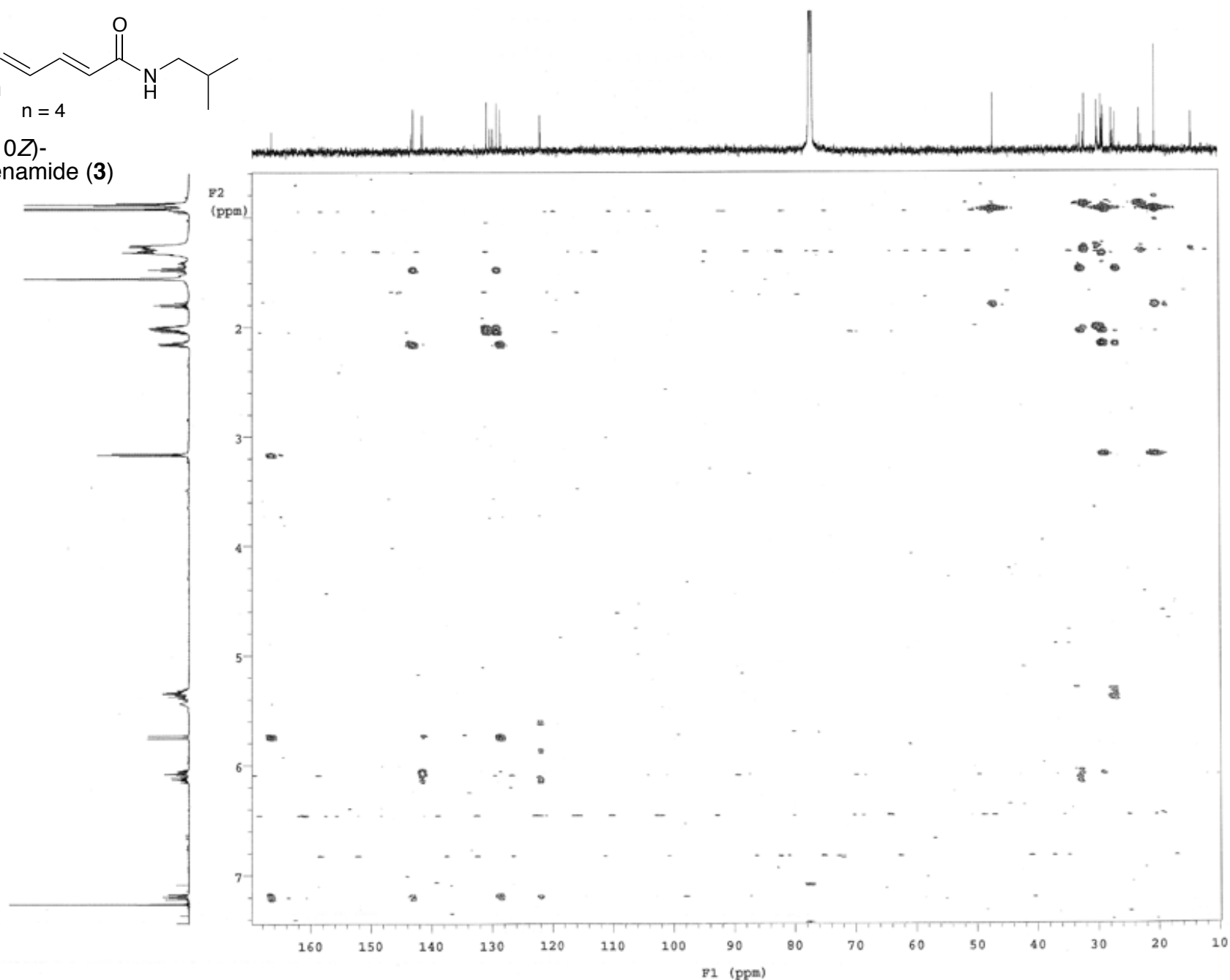
HMQC of N -isobutyl-(2 E , 4 E , 10 Z )-hexadeca-2,4,10-trienamide ( 3 )
