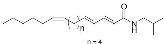
N -isobutyl-(2 E , 4 E , 10 Z )-hexadeca-2,4,10-trienamide ( 3 )
