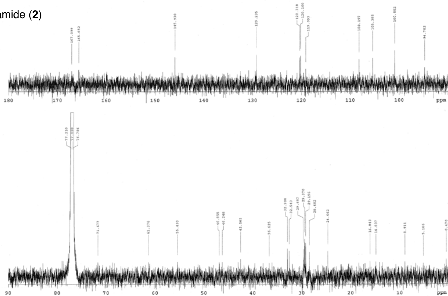
^{13}\text{C} NMR data of (2 E , 12 E )-pipertridecadienamide ( 2 )
