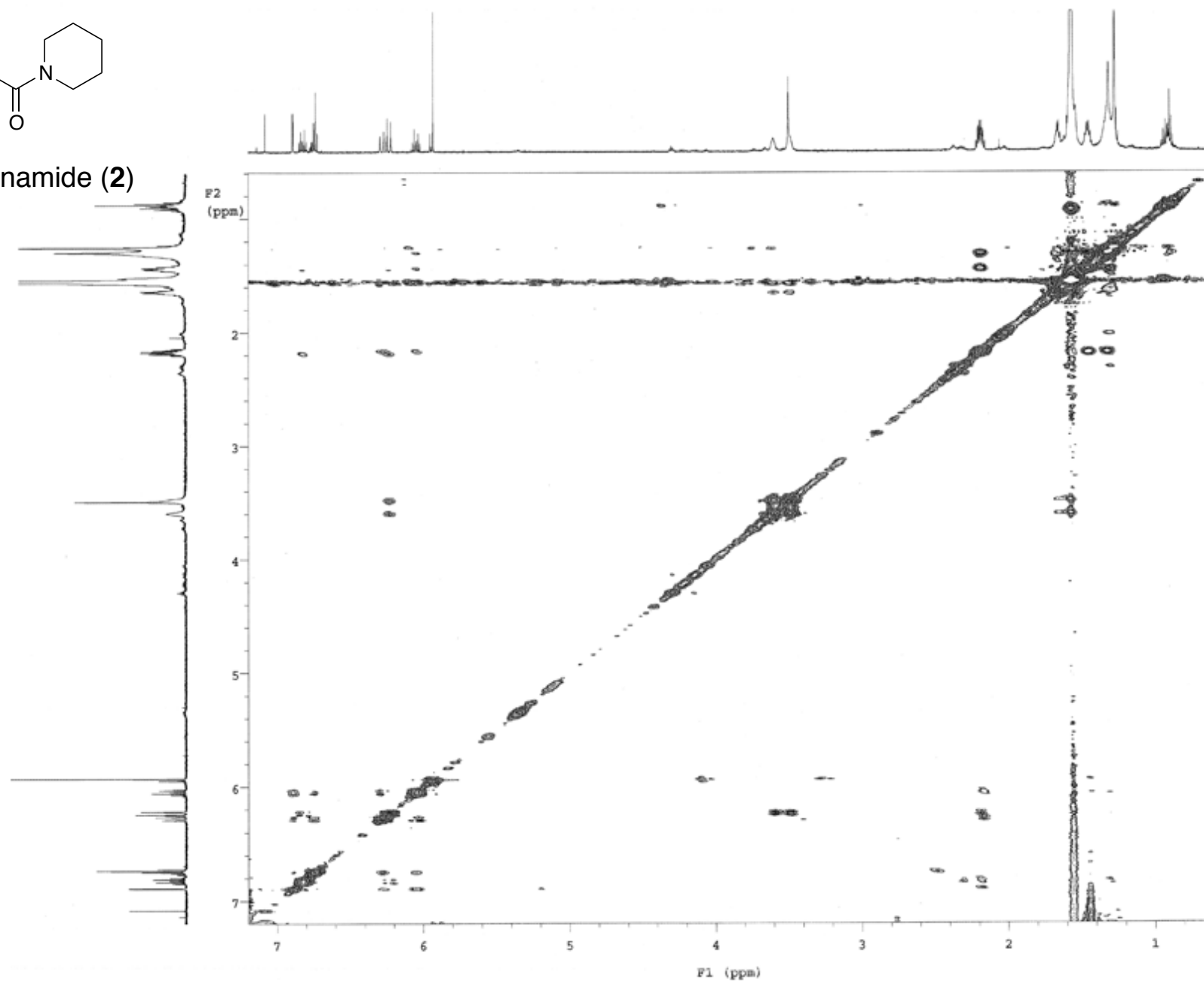
NOESY of (2 E , 12 E )-pipertridecadienamide ( 2 )
