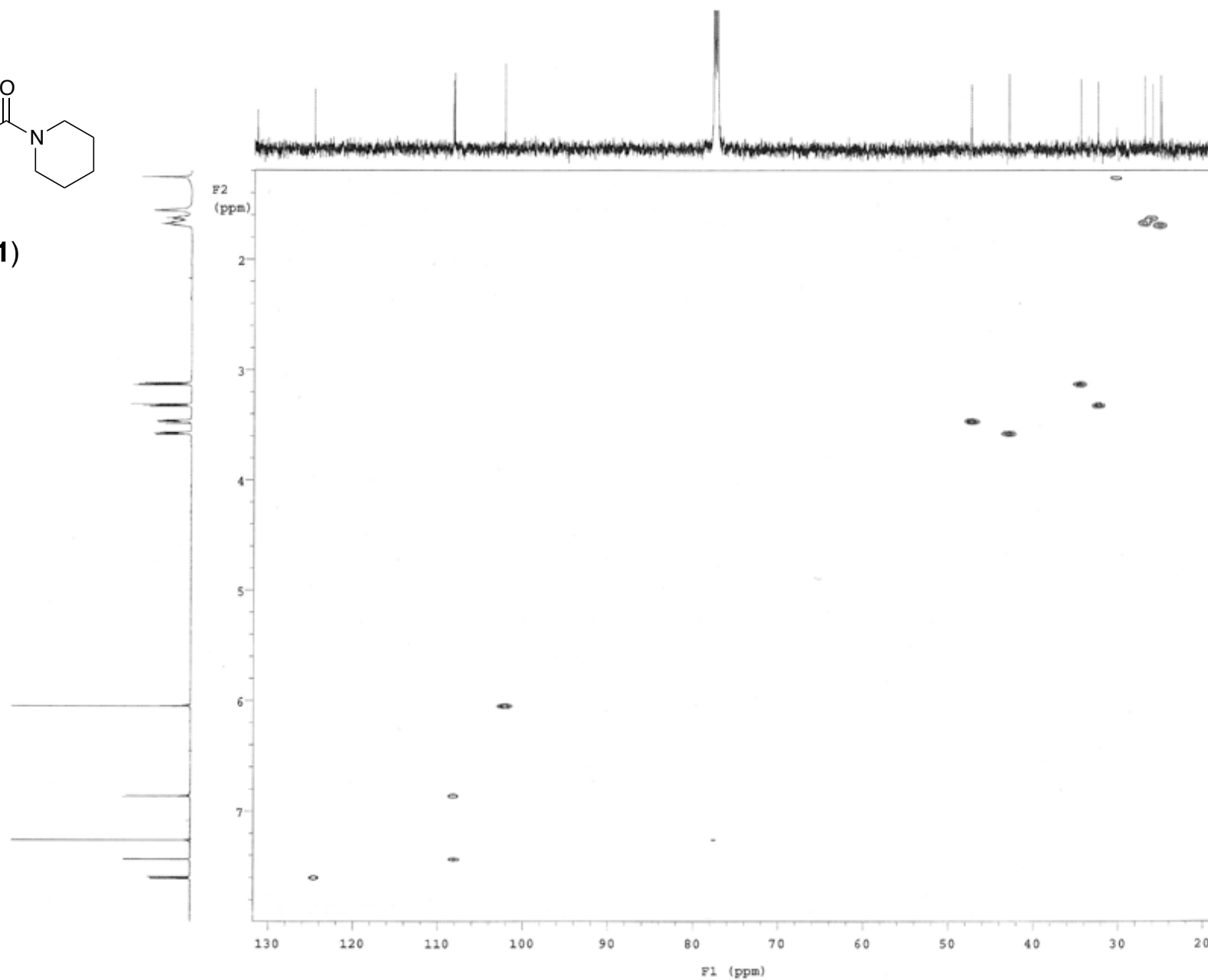
HMQC of piperone (1)
